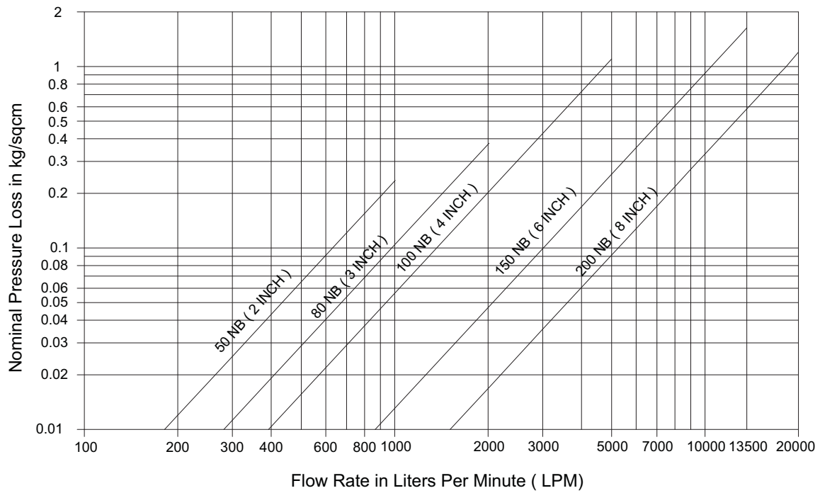
Nominal Pressure Loss vs Flow - Deluge Valve ( Model-A)
